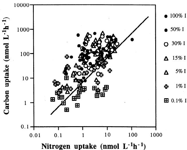
Figure 4. Log plot of carbon and nitrogen uptake rates by phytoplankton as a function of irradiance. Irradiance (I) fields are a percentage of the surface level; total nitrogen uptake is nitrate plus ammonium assimilation. Line shows Redfield ratio for comparison (C:N = 6.6).
